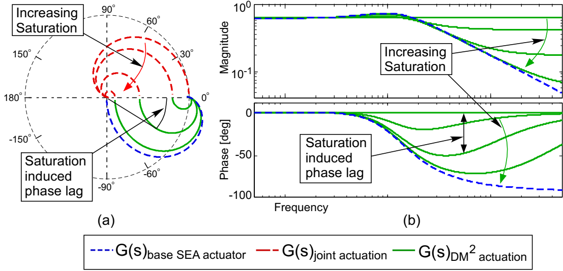
Figure 12: Breakdown of perfect torque source due to saturation (a) Base, joint (with saturation), and resulting DM 2 actuator torque magnitude vs phase polar plot (b) Bode plot of DM 2 actuator torque with joint actuator saturation
