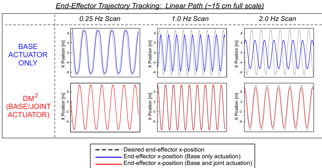
Figure 24: End effector position tracking control experimental results.
