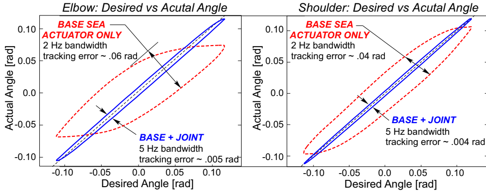
Figure 23: Comparison of position tracking performance using base actuation only with combined base and joint actuation ( DM^2 )
