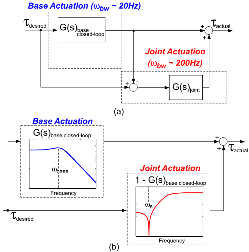
Figure 10: (a) DM 2 actuation control structure ( G(s)_{base-closed-loop} : Base actuator closed loop transfer function. G(s)_{joint} : Joint actuator transfer function) (b) Equivalent parallel structure
