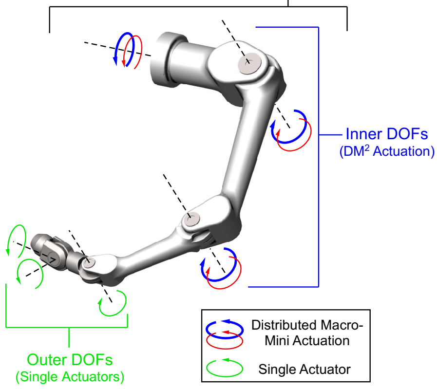
Figure 25: Implementation of DM 2 actuation for multi-DOF manipulator
