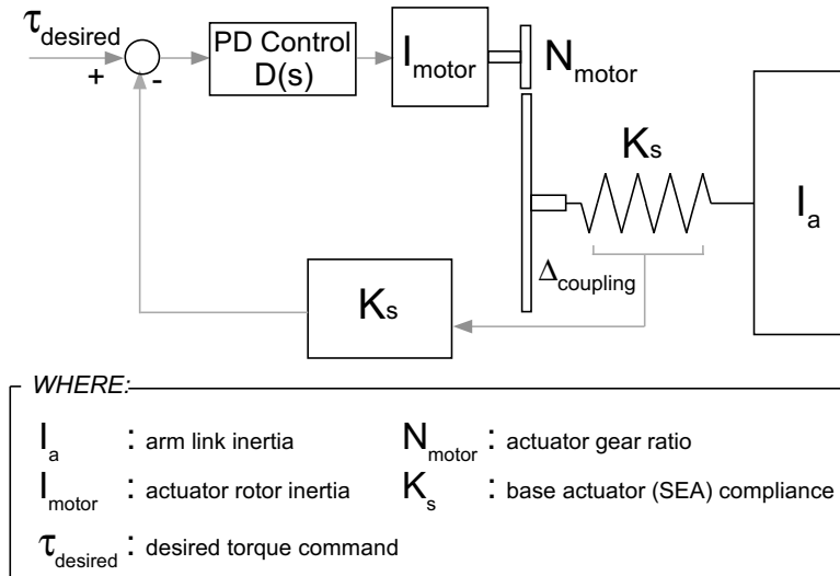
Figure 4: Series elastic actuation (SEA) topology
