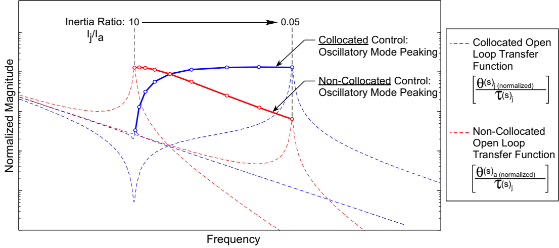
Figure 19: Variation of peaking amplitude for collocated and non-collocated position control for varying motor to load inertia ratios, I_j/I_a
