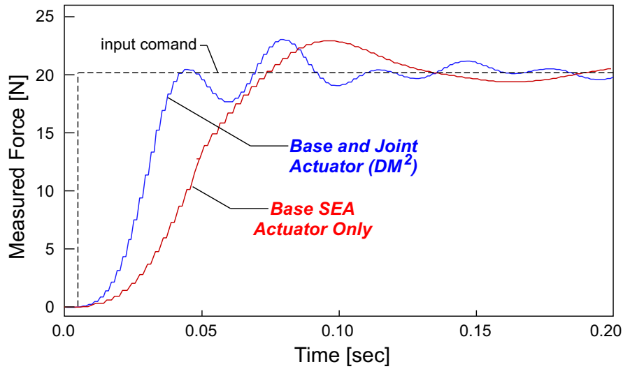
Figure 22: Open-loop end-effector force (step) response.
