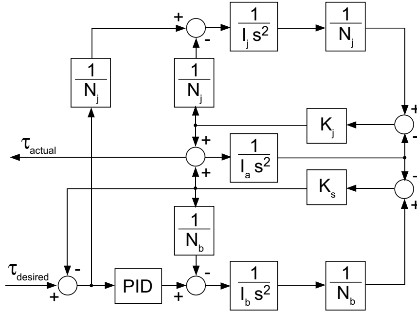
Figure 14: Augmented DM 2 actuation and control block diagram representation (single DOF). Joint actuator drive-train compliance included.
