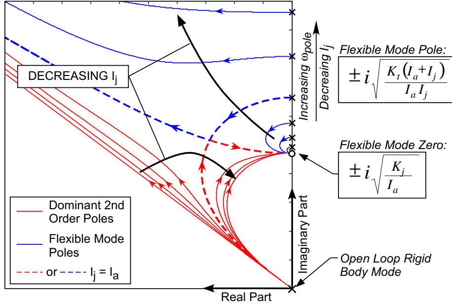
Figure 18: Symmetric root locus of collocated position control system with shaft compliance
