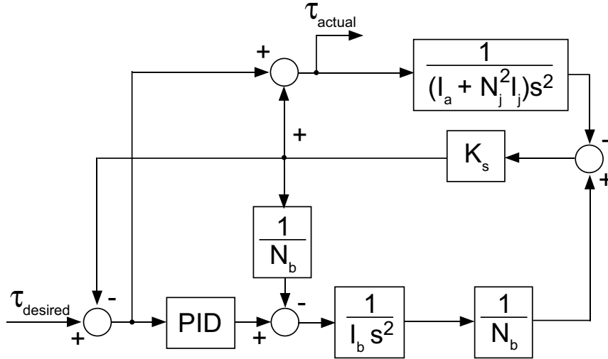
Figure 9: DM 2 Actuation and control block diagram representation (single DOF)
