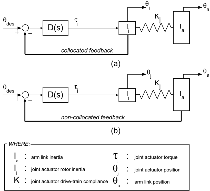
Figure 16: Spring-mass model of joint actuator and driven link Inertias (a) Collocated control (b) Non-collocated control
