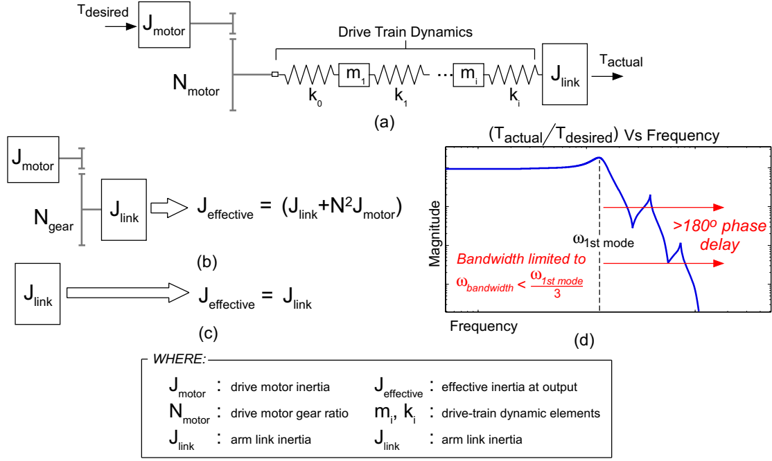
Figure 2: (a) Robotic manipulator compliant drive-train mass-spring model (b) Low frequency effective inertia approximation (c) High frequency effective inertia approximation (d) Open-loop T_{\text{actual}} / T_{\text{desired}} magnitude vs frequency
