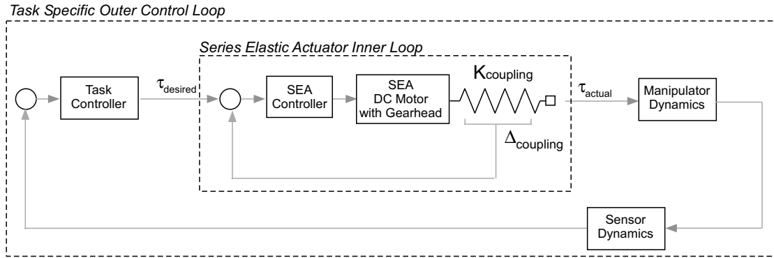
Figure 5: Nested series elastic actuation and outer task control loops
