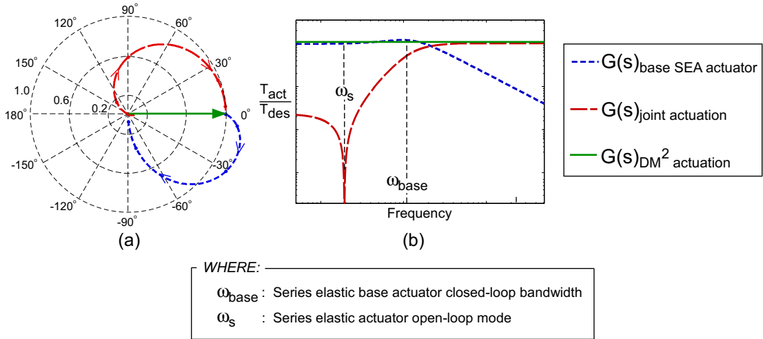
Figure 11: (a) Perfect torque source: Base, joint, and combined DM 2 actuator torque magnitude vs phase polar plot (b) Near perfect torque source: Base, joint, and combined DM 2 actuator torque magnitude vs frequency
