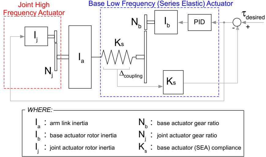
Figure 8: DM 2 Actuation and control topology (single DOF)
