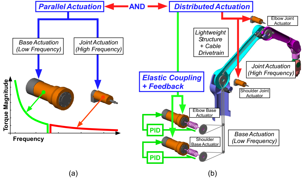
Figure 6: Distributed Macro-Mini (DM 2 ) actuation approach (a) Partition of torque into low and high frequency (parallel) components (b) Distributed actuation: Large, low frequency actuators are located at base. Small, high frequency actuators are located at the joints
