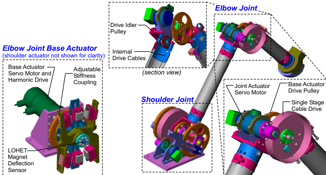
Figure 20: Two axis DM^2 prototype
