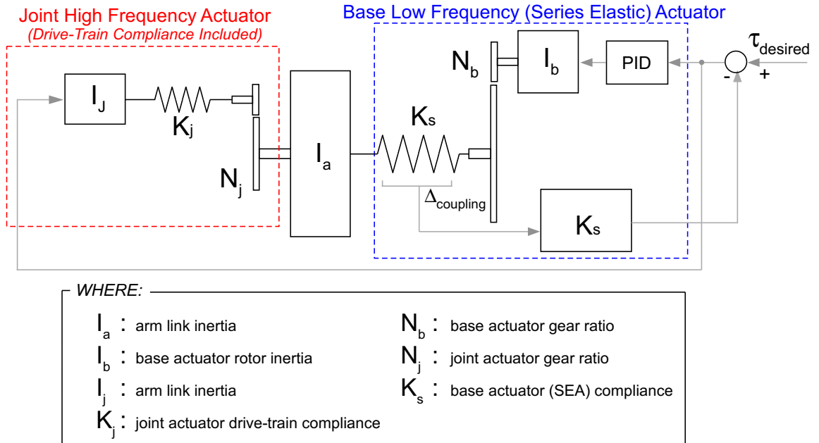
Figure 13: Augmented DM 2 actuation and control topology (single DOF). Joint actuator drive-train compliance included.
