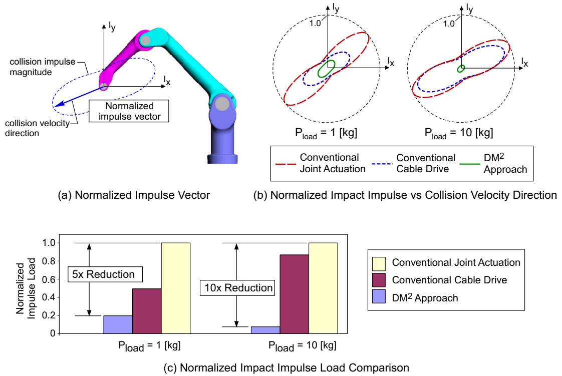
Figure 21: Comparison of impulse load due to impact for various actuation concepts. (a) Normalized impulse vector: Impulse due to collision of manipulator end effector with rigid object. Impulse magnitude changes with angle due to variation of end-effector effective inertia as a function of impact direction. (b) Normalized impact impulse vs collision velocity direction for various actuation concepts and values of end-point load ( P_{load} ). (c) Comparison of normalized impact impulse load for various actuation concepts and values of end-point load ( P_{load} ). Impulse values are normalized by impact velocity and maximum effective inertia.
