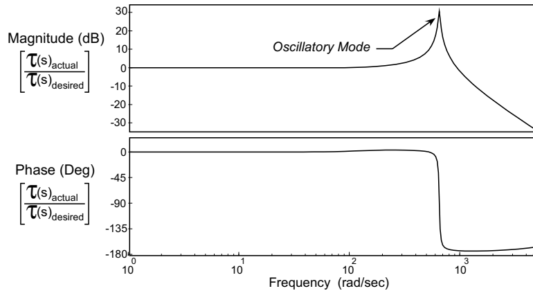
Figure 15: Bode plot of augmented DM 2 actuation and control block diagram representation (single DOF). Joint actuator drive-train compliance included.
