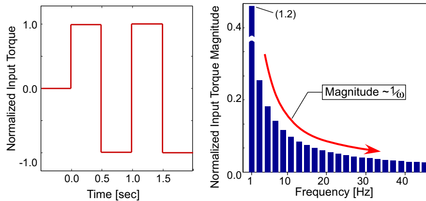
Figure 7: Torque vs frequency: 1 Hz square wave
