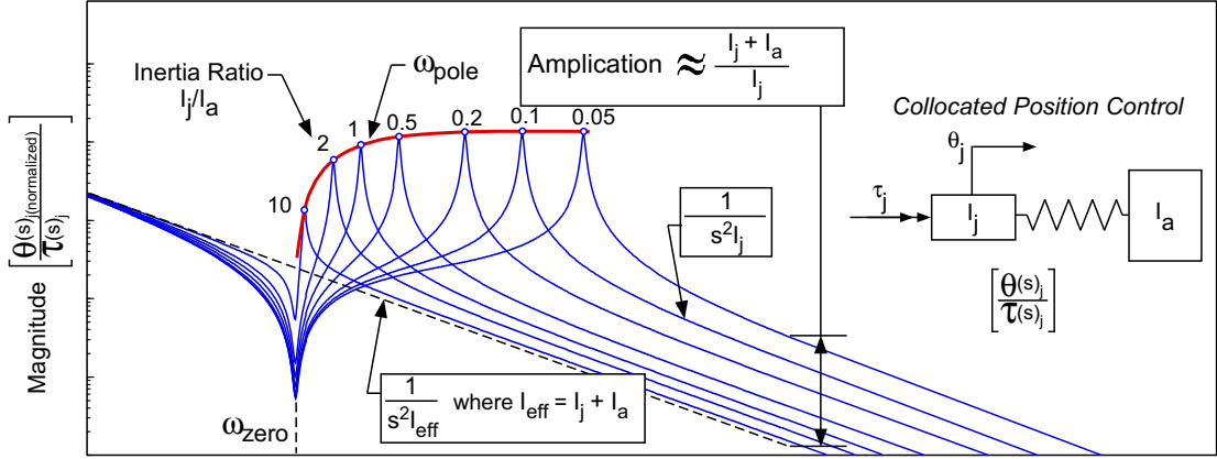
Figure 17: Open loop transfer function of collocated motor position control: Amplification of oscillatory pole due to mismatched actuator-link inertia
